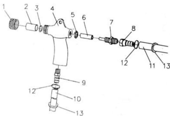
Abb. 14: Blaspistole
