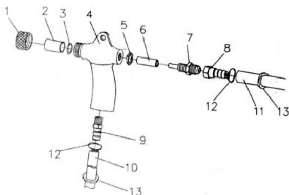
Abb. 6: Blaspistole
