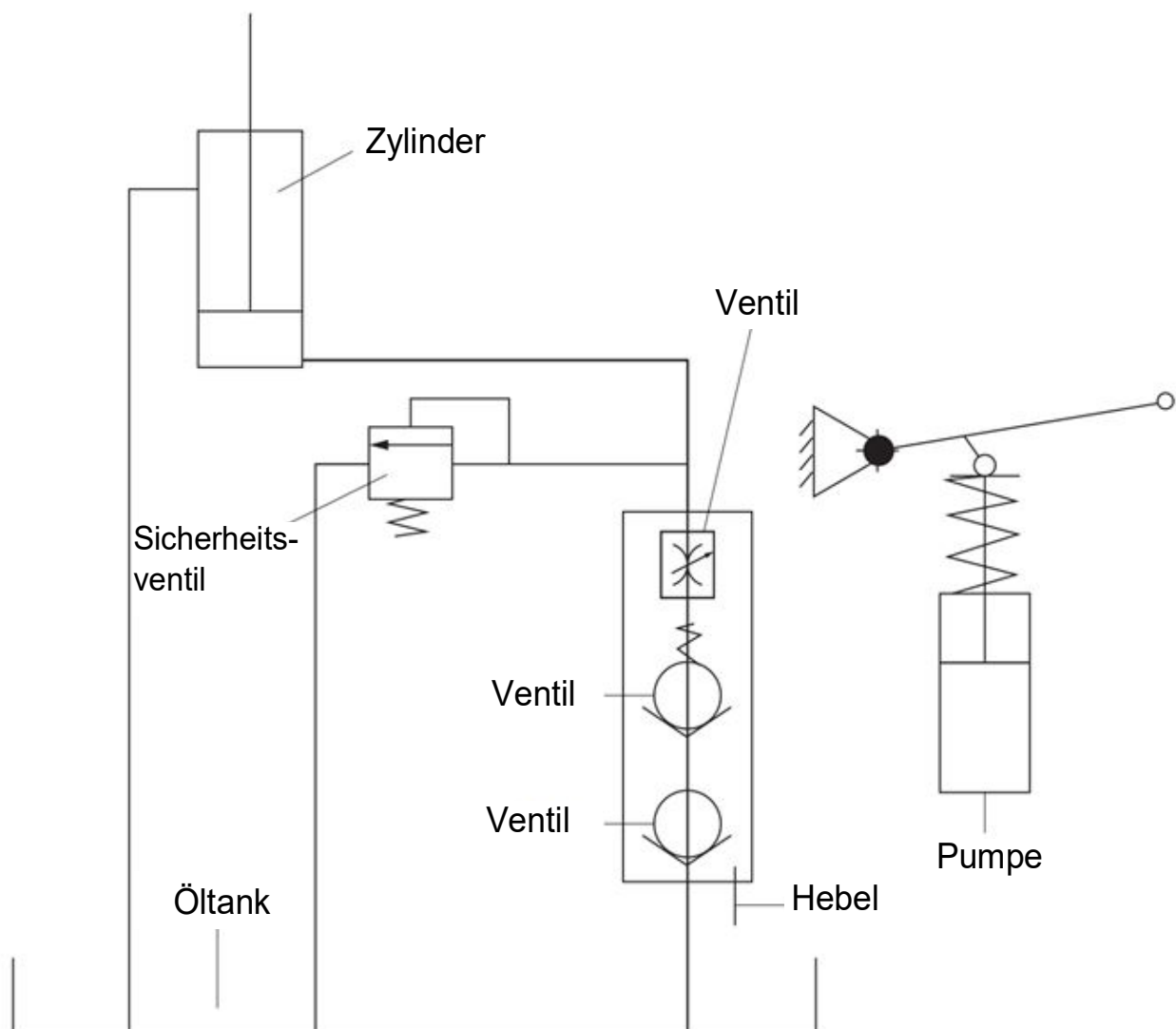
Abb. 11-1: Hydraulikplan
